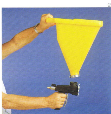
Hopper spray gun can be quickly and easily disassembled (e.g. for cleaning).
